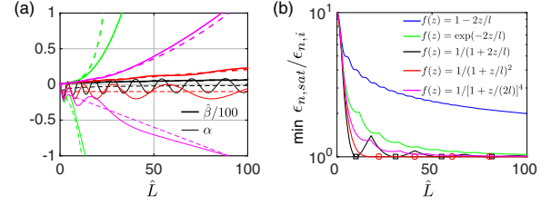
FIG. 2. The performance of the matching plasma with different density profiles. (a) The evolution of the CS parameters when \hat{l} = 5 . Thick and thin lines represent \beta functions and \alpha functions. The colors correspond to the profiles listed in (b). Solid lines are from the analytical solutions and the dashed lines are based on adiabatic approximations where \hat{\beta} = f(z)^{-1/2} . (b) For each \hat{L} , \hat{l} is scanned to find the optimized value. The parameters are \hat{\beta}_i = 1 , \alpha_i = 0 , \hat{\beta}_{\text{goal}} = 20 , \alpha_{\text{goal}} = 0 , and the case is of a transition from a PBA to a magnetic optics.
