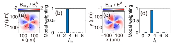
FIG. 6. Simulation results of magnetic or optical vortex generation through the collision of a \text{LG}_{0,1} \text{CO}_2 laser with a second-order helical IF. (a) and (c) show the slice plots of the magnetic vortex B_{m,y} and optical vortex E_{t,x} , respectively. (b) and (d) show the azimuthal decomposition results of the magnetic [corresponding to (a)] and optical [corresponding to (c)] vortices at a radius of r = 100 \mu\text{m} (dashed circle), respectively.
