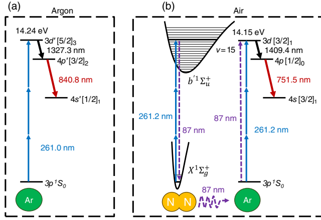
FIG. 1. Relevant transitions of three-photon excitation and cascade lasing in pure Ar and atmospheric air. (a) In pure Ar, the Ar atoms are excited by the 261 nm pump pulse to the 3d'[5/2]_3 state (14.24 eV) and emit first lasing at 1327.3 nm and second lasing at 840.8 nm. (b) In atmospheric air, the N_2 molecules are excited to the b'^1\Sigma_u^+ ( v = 15 ) state (14.1551 eV) by the 261.2 nm pump pulse, and emit third-harmonic photons at 87 nm, which is reabsorbed by the surrounding Ar atoms so that the Ar atoms are excited to the 3d[3/2]_1 state (14.1525 eV) and then emit first lasing at 1409.4 nm and second lasing at 751.5 nm. Note that the center wavelengths of the pump are slightly different: 261.0 nm (Ar) vs 261.2 nm (air) to optimize the pumping of the three-photon resonance.
