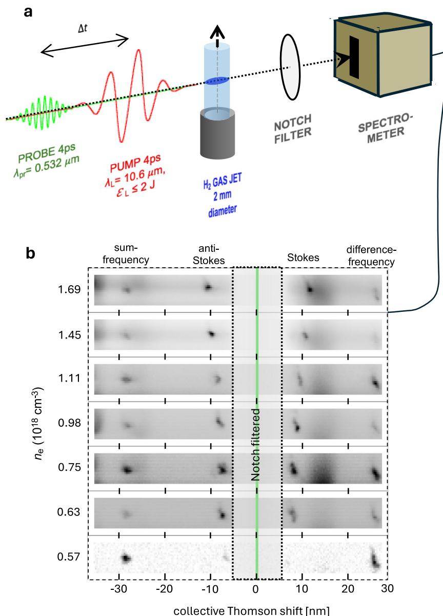
Fig. 2 | Collective Thomson Scattering probing of SM wakes. a Schematic experimental setup with green probe pulse co-propagating at delay \Delta t behind \text{CO}_2 pump pulse. b Spectra of forward-scattered probe light for P_L = 0.5 TW and \Delta t \approx 0 , for
