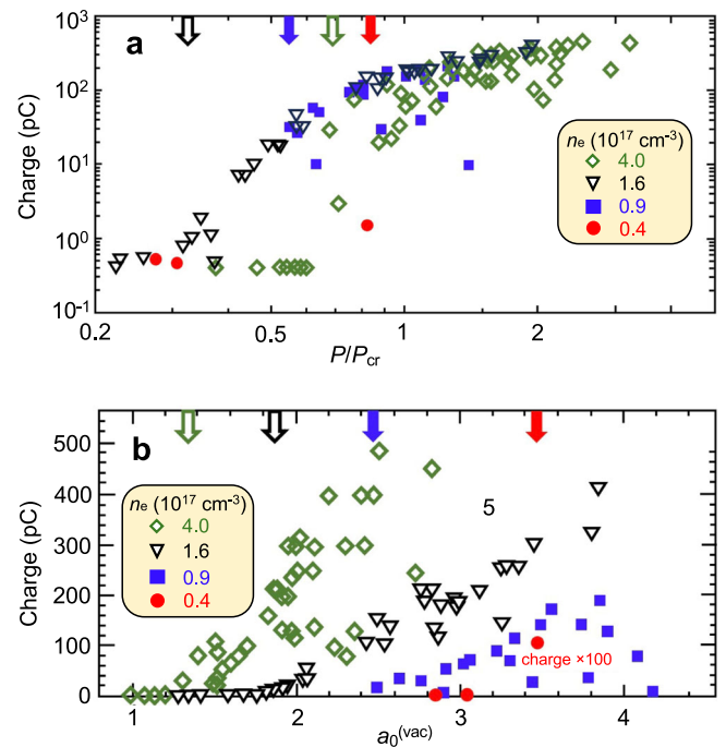
Fig. 6 | Charge of accelerated electron bunches. a Total charge of > 1 \text{ MeV} electrons vs. normalized peak power P/P_{cr} of \sim 2 \text{ ps} laser pulses driving LWFA in plasma of 4 densities in the range 0.4 \times 10^{17} \leq n_e \leq 4 \times 10^{17} \text{ cm}^{-3} as per key. b Data from a re-plotted as a function of a_0^{(vac)} . Color-coded arrows at top of a , b : electron appearance thresholds for each n_e .
