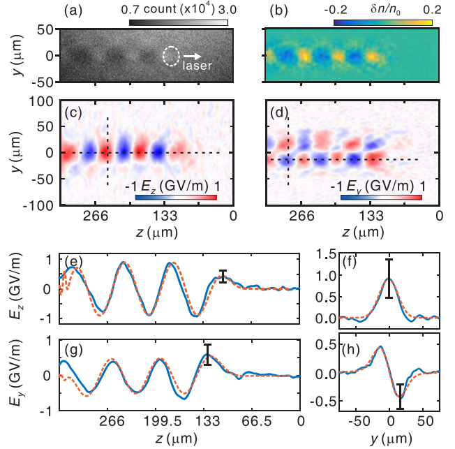
FIG. 2. Snapshot of the wake, the deduced electric field structure of the wake, and comparison with simulations. (a) Raw image of the probe density n . (b) Density modulation \delta n/n_0 . (c) and (d) The (y, z) plot of the reconstructed E_z and E_y field, respectively. (e) and (f) The axial and transverse ( z = 242 \mu\text{m} ) lineouts of E_z , respectively. (g) and (h) The axial (at y = -10 \mu\text{m} ) and transverse ( z = 300 \mu\text{m} ) lineouts of E_y . The blue solid lines show the experimental data, while the red dashed lines are from simulations. The transverse lineouts are taken at positions where the agreement between the simulations and the experiment is the closest. The error bars arise from the fluctuating energy, pulse width, and correlated divergence of the probe beam.
