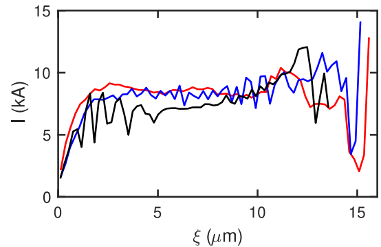
FIG. 5. Current profile of the injected beam. The ramp parameters are the same as those in Fig. 4. The red, blue, and black lines correspond to ramp length of 5, 10, and 25 c/\omega_p , respectively.
